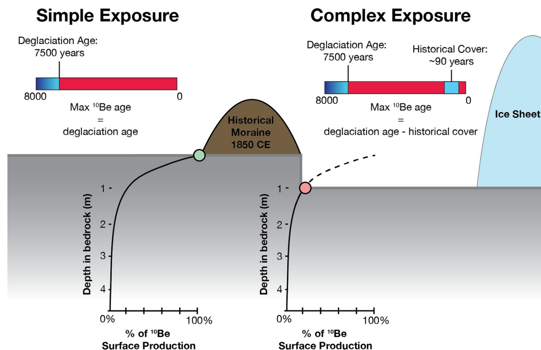
Figure 4. Schematic of the Jakobshavn Isbræ forefield describing how erosion rates are derived from the measured ^{10}\text{Be} concentrations. The bedrock outboard (left) of the historical moraine experienced only one continuous period of exposure during the Holocene, as shown in the timeline, so a surface sample collected at the light green circle would have an apparent exposure age that reflects the true deglaciation age of the site. The bedrock inboard (right; sample location similar to that of Young et al. (2016)) of the moraine, shown in pink, has a complex exposure history, including the \sim 90 years of ice cover at the end of the Holocene. During this most recent period of ice cover, any subglacial erosion would remove the upper portion of the ^{10}\text{Be} depth profile in the bedrock, accumulated from previous exposure, so the measured ^{10}\text{Be} concentration would be lower than the true exposure age. For the sake of illustration, a surface sample collected at the pink circle experienced 1-m of subglacial erosion during historical cover, and therefore its ^{10}\text{Be} concentration would be 20% of the expected concentration.
