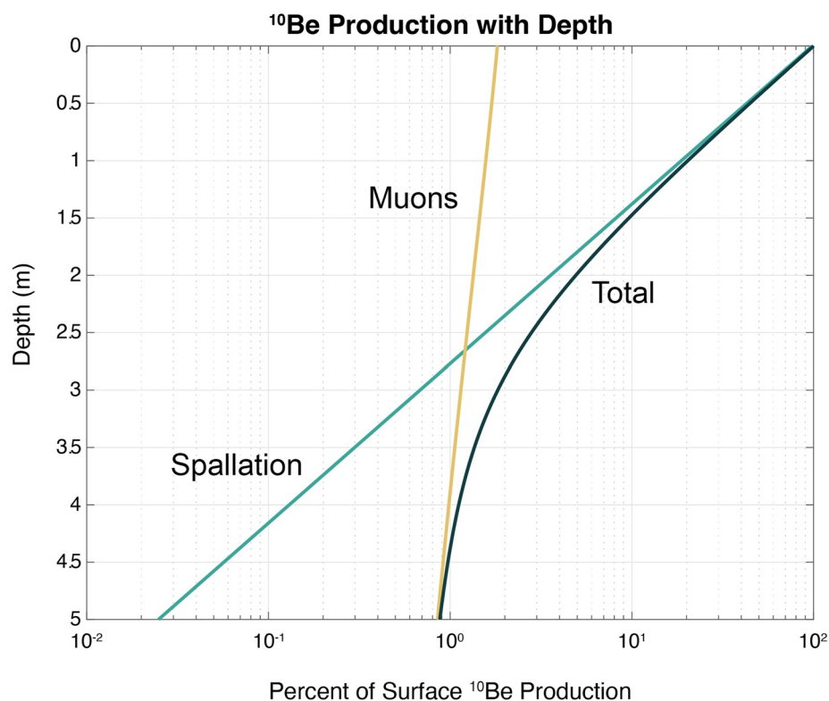
Figure 3. ^{10}\text{Be} production profile shown as percent of surface production at sea-level high latitude. Although the production rate varies with geomagnetic latitude and elevation, the relative proportion of production by muons and spallation is similar at Jakobshavn Isbræ, with \sim 1\% production by muons at the surface. Note that by \sim 2.5 m depth, muon production exceeds spallation production.
