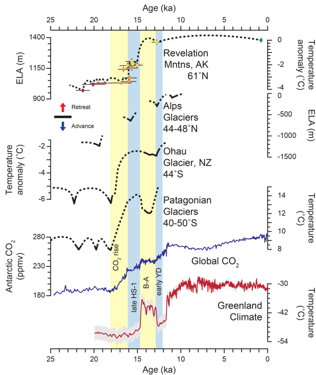
Figure 7. Comparison of the Revelation Mountains retreat chronology with Southern Hemisphere and Alps glacial retreat, as well as global and regional climate forcing mechanisms. Top to bottom: the Revelation Mountains ELA-based temperature curve (this study), composite ELA reconstructions from the Alps (Ivy-Ochs, 2015), temperature curve from Ohau Glacier, NZ (Putnam et al., 2013), composite temperature curve from Patagonian glaciers (Denton et al., 1999; Strelin et al., 2011), composite atmospheric CO 2 concentrations from Antarctic ice cores (Bereiter et al., 2015), and Greenland-wide average mean annual temperature from ice cores (20–11 ka; Buizert et al., 2014, 11–0 ka; Kobashi et al., 2017).
