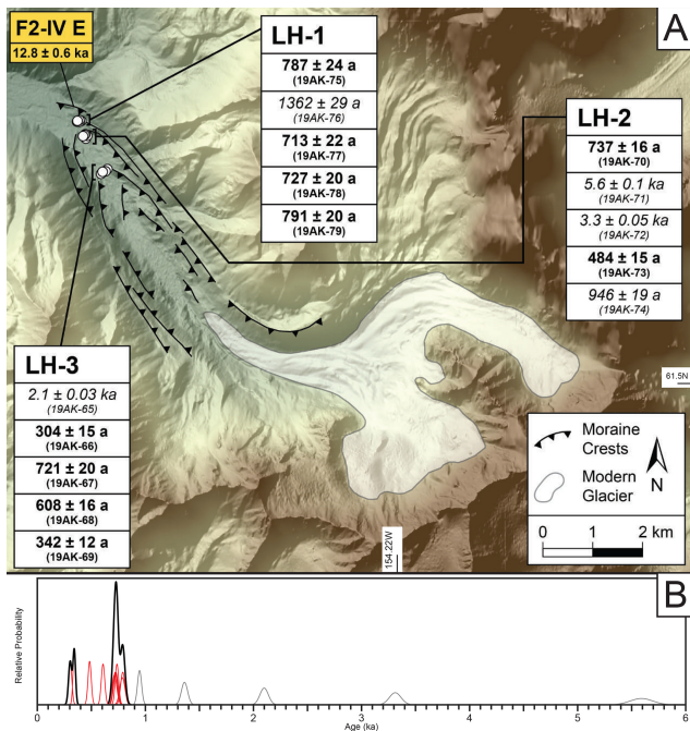
Figure 2. (a) Shaded relief map of the modern North Swift River valley glacier and late Holocene moraines with ^{10}\text{Be} ages displayed. Samples listed in italics are suspected outliers. The age for the F2-IV E moraine segment is from Tulenko et al. (2022). Map source: 5 m resolution IFSAR Alaska DEM product available from the USGS. (b) Normal probability density functions (PDFs) for individual ages are in red and summed PDFs for the two clusters of ages around 750 and 320 a are in black. Ages older than expected and well beyond 2 standard deviations from other ages in the dataset are in gray.
