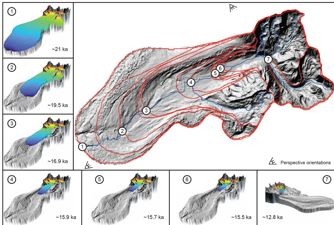
Figure 6. Plan view of the North Swift River valley and reconstructed glacier extents in the main panel. Outlines of every glacier surface and extent reconstructed in this analysis (in red). Blue lines are the flowlines reconstructed on the resampled, lower-resolution DEM. In the insets are 3D visualizations of reconstructed glacier surfaces. ELA reconstructions at each glacier position viewed in oblique 3D with 4\times vertical exaggeration. Each number in the main panel corresponds to the toe of the glacier position reconstructed in each inset panel. Glacier surfaces 1–6 are viewed from the perspective in the bottom left corner of the main panel, and glacier surface 7 is viewed from the perspective near the top right.
