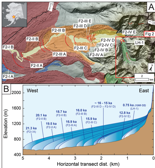
Figure 1. (a) Moraine map of the North Swift River valley with reconstructed moraine positions denoted with red lines ( n = 15 ). Color overlays denote broad morphostratigraphic equivalence of landforms and are arranged as darker shades being stratigraphically older than lighter shades. Blue shades are MIS-4-age moraines, brown-red shades into yellow shades are LGM and deglacial moraines, and green are Holocene-age moraines. Inset: starred location of the Revelation Mountains in Alaska. (b) Schematic of alpine glacier retreat in the North Swift River valley that includes moraine ages reported here and in Tulenko et al. (2022). Panel (a) source: ArcticDEM product available from the University of Minnesota Polar Geospatial Center. Inset map source: IBCAO product available from GEBCO.
