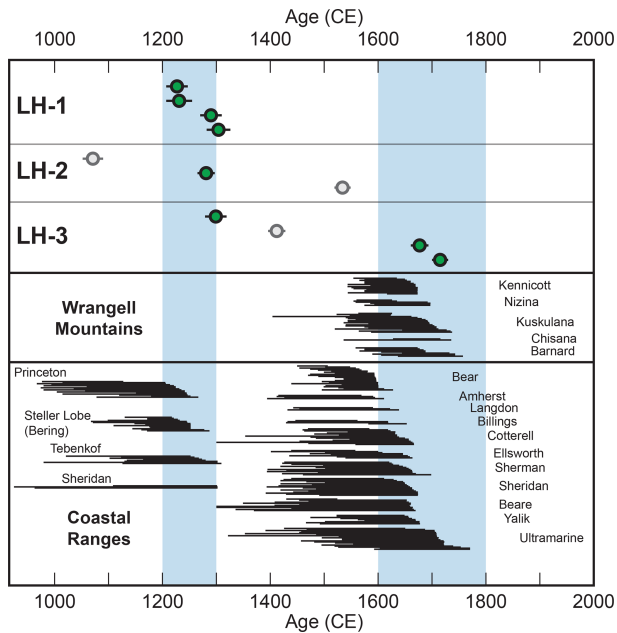
Figure 5. Comparison of late Holocene moraine ages (green dots; gray dots are outliers) with tree-ring-based southern Alaska glacial fluctuations (black bars; Barclay et al., 2009). Light blue vertical bars indicate periods of moraine deposition in the Revelation Mountains (upper panel) and tree-kill dates signifying glacier culminations in southern Alaska (lower panels) at \sim 1200 – 1300 CE and \sim 1600 – 1800 CE. See Fig. 4 for geographic locations of tree-kill dates.
