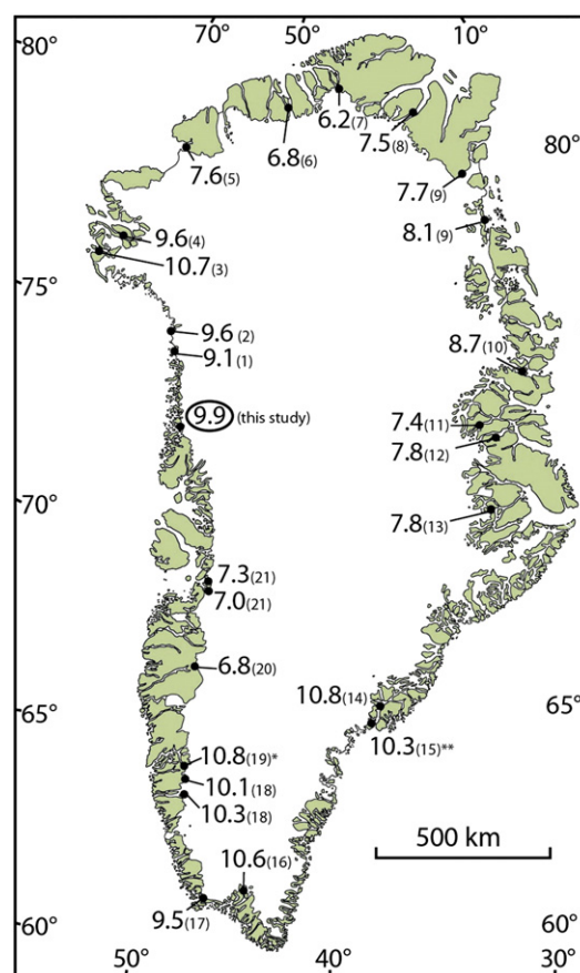
Figure 6. Map of Greenland showing the distribution of the closest ages ( ^{14}\text{C} and ^{10}\text{Be} ) to the historical ice limit around the Greenland Ice Sheet. Ages are presented in ka; see original reference for age uncertainty and other details. 1: Bennike (2008); 2: Fredskild (1985); 3, 4, 11: Weidick (1978); 5: Bennike (2002); 6: Kelly and Bennike (1992); 7: Landvik et al. (2001); 8: Funder (1982); 9: Bennike and Weidick (2001); 10: Weidick (1977); 12: Håkansson (1976); 13: Funder (1978); 14: Hughes et al. (2012); 15: Roberts et al. (2008); ^{10}\text{Be} ages adjusted for production rate to be consistent with more recent studies (14, 18, 20, 21); 16: Larsen et al. (2011); 17: Kaplan et al. (2002); 18: Larsen et al. (2013); 19: Weidick et al. (2012); the 10.8 ka age is from a bivalve that was reworked into a moraine assigned to 8.3–8.1 ka, and is interpreted as indicating initial deglaciation prior to a re-advance); 20: Levy et al. (2012); 21: Young et al. (2013).
