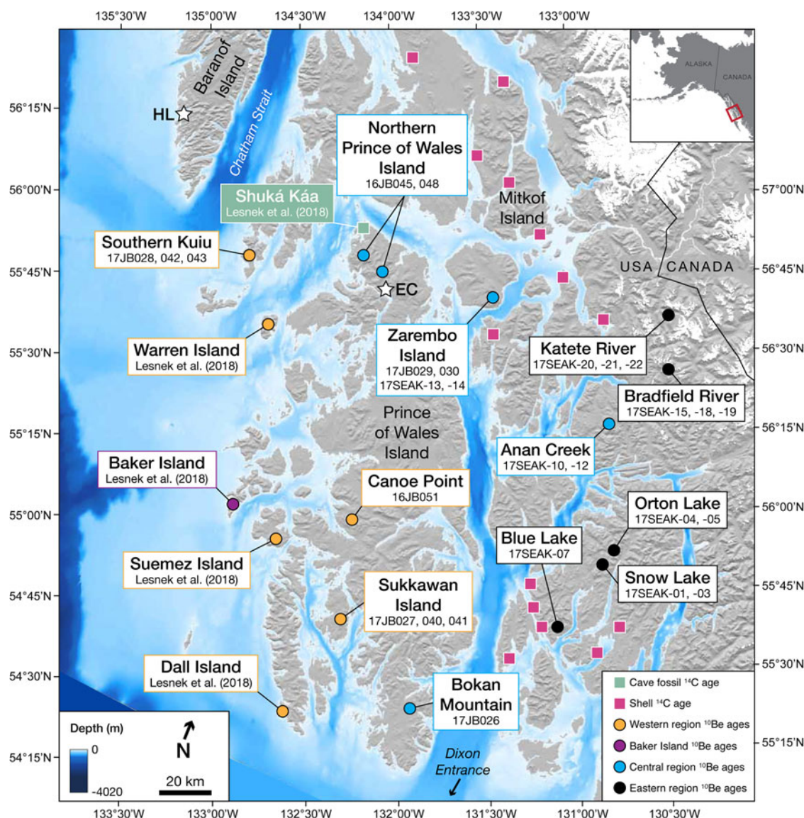
Figure 2. Map of study area. 10 Be sampling sites are indicated by the dots. Sites are color coded, where yellow = western region, purple = Baker Island (local glaciers), blue = central region, and black = eastern region. 14 C sampling locations are indicated by squares. Green = Shuká Káa cave (Lesnek et al., 2018), pink = shell-bearing raised marine sediments. White stars indicate locations of previous work mentioned in the text. HL = Hummingbird Lake (Ager et al., 2019), EC = El Capitan Cave (Wilcox et al., 2019). Modern glacier extents (white) are from version 6 of the Randolph Glacier Inventory (NSIDC, 2005, updated 2018). (For interpretation of the references to color in this figure legend, the reader is referred to the web version of this article.)
