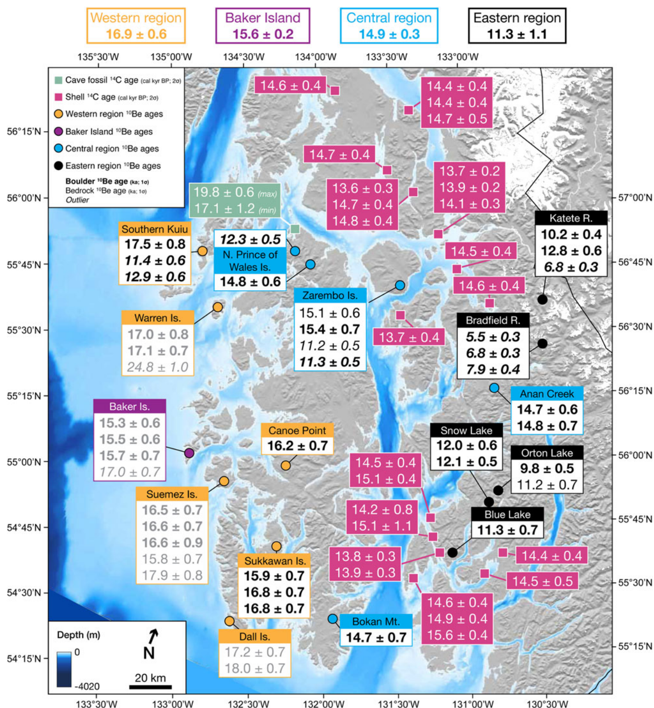
Figure 6. Map of Southeast Alaska with deglaciation chronology. Ages are color coded by type and region. 14 C ages from Shuká Káa (Lesnek et al., 2018) are shown in green boxes with white text. Minimum-limiting 14 C ages from raised marine sediments are shown in pink boxes with white text. All 14 C ages are calibrated and shown at 2 SD uncertainty. 10 Be ages from this study are shown in white boxes with black text. Previously published 10 Be ages (Lesnek et al., 2018) are indicated with gray text. Boulder ages are in bold text, bedrock ages are in normal text. All 10 Be ages are color coded by region: yellow = western region, purple = Baker Island (local glaciers), blue = central region, and black = eastern region. Outliers are indicated by italic text. All 10 Be ages are shown at 1 SD external uncertainty. Average 10 Be ages for each region (mean ± 1 SD) are shown at the top of the image. (For interpretation of the references to color in this figure legend, the reader is referred to the web version of this article.)
